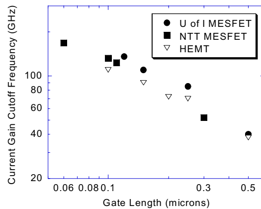
Fig. 6 Comparison of current results to AlGaAs/GaAs HEMTs and NTT MESFETs
