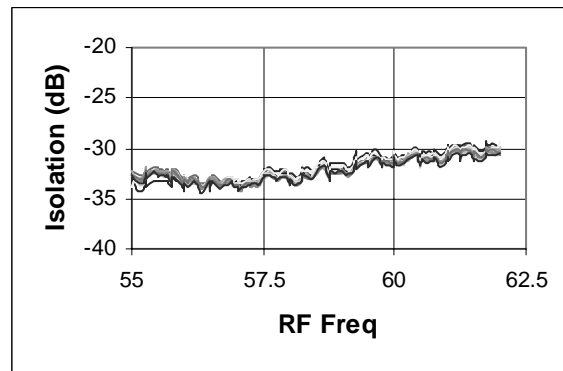
Fig. 7. Output Port-Port Isolation, SDH126
