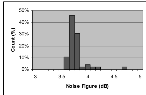
Fig. 2. ALH382 Noise Figure Statistics @ 60 GHz
