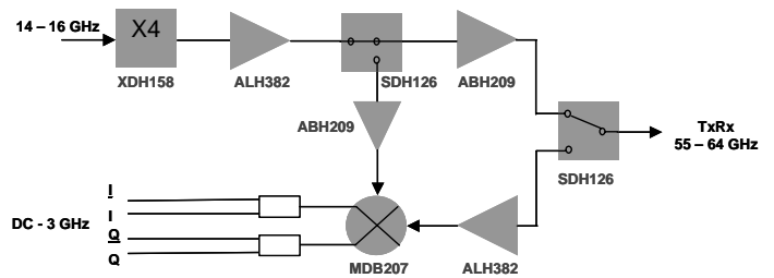
Fig. 1. V-Band Transceiver
