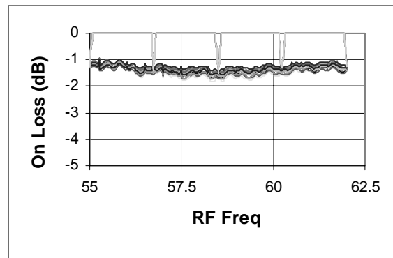
Fig. 6. Insertion Loss, SDH126
