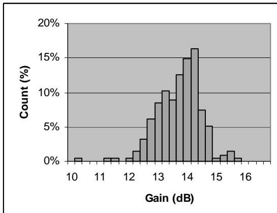
Fig. 10. ABH209 Power Amplifier Gain at 60GHz
