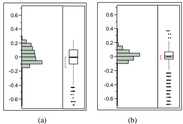
Figure 5. The distribution of V_T (threshold voltage measured at V_{DS} of 10 V and I_{DS} of 1 mA/mm) from the group average value (a) before and (b) after the improvement. The standard deviation was improved from 0.12 to 0.09 V.
